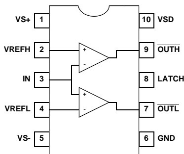
EL5283 (10-PIN MSOP) TOP VIEW
